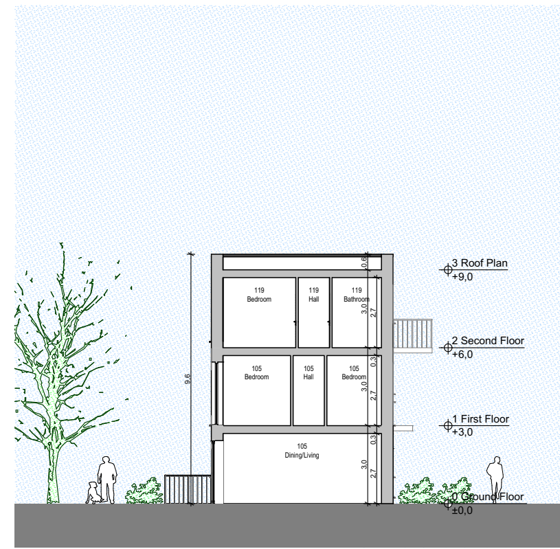
Section 1 - 1 1:200
